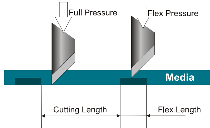
FIG 3-3 FLEXCUT PRINCIPLE
