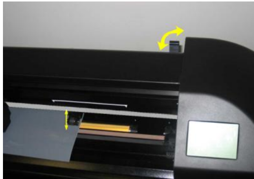
FIG 1-17 PINCH ROLLER LEVER
