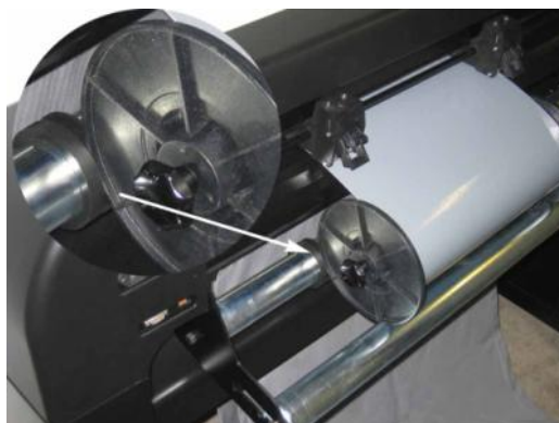
FIG 1-19 POSITION MEDIA FLANGE ON CUTTER
