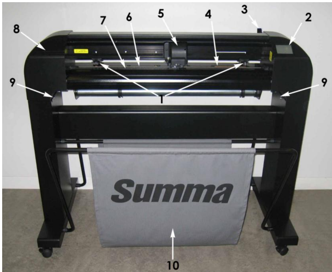
FIG 1-10 S CLASS™ CUTTER, FRONT VIEW
