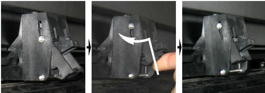
FIG 1-16 REDUCING PRESSURE
